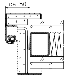
Zarge "ZG 68/76"
