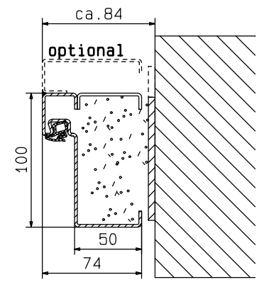
Zarge "ZG 68/76"
