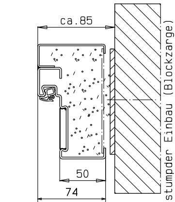
Zarge "ZNG 68/76"
